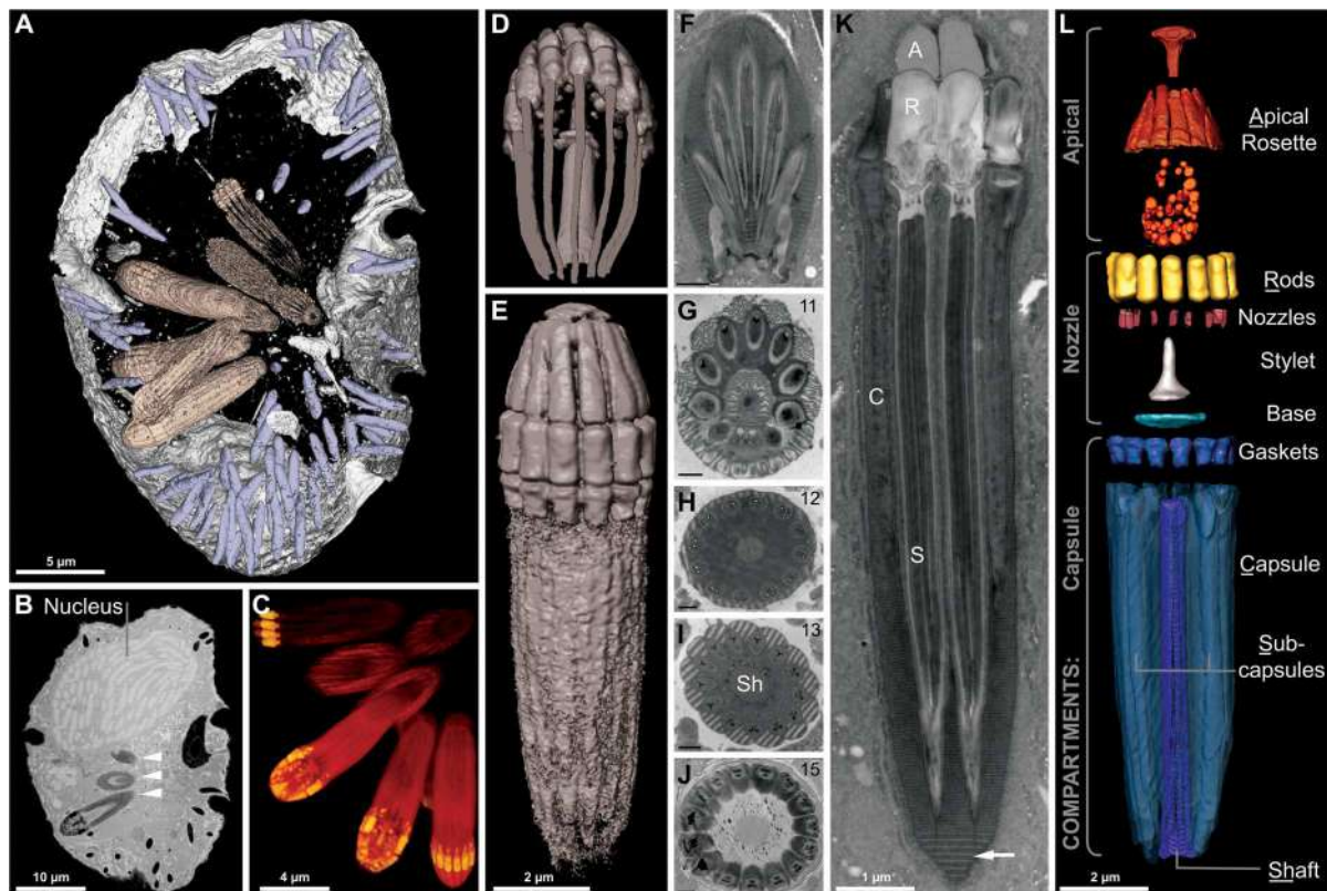
Fig. 4. Reconstruction of the nematocysts in Nematodinium sp. (A to E) Images derived from single-cell FIB-SEM. (A) Partial reconstruction of a cell with nematocysts shown in beige and mucocysts shown in purple. (B) Longitudinal FIB-SEM section through a cell showing the nucleus and nematocysts (arrowheads). (C) 3D maximum intensity projection showing a battery of nematocysts. (D) 3D tilted reconstruction of a nematocyst. (E) Longitudinal reconstruction of a nematocyst. (F to K) Single-cell TEM micrographs of a nematocyst in oblique section (F), cross section (G to J), and longitudinal section (K) showing the striated material (arrow) and variable symmetries across different nematocysts, with the number of subcapsules printed in the upper right corner. (L) A virtual dissection of the nematocyst components. Brackets indicate the membrane-bound compartments bounding the components indicated. (F) to (J) scale bar, 500 nm.
